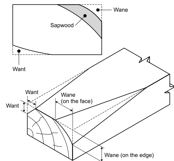
Figure B3.6 Wane, want and sapwood
