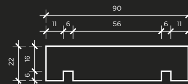
Cover Batten/Fascia
