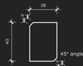
Eaves Mould
