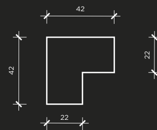
External Corner
